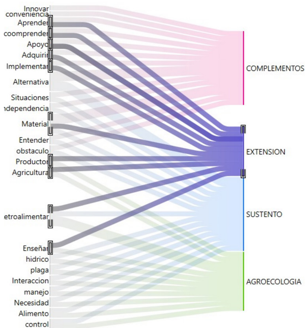
Figure 5. Sankey diagram
